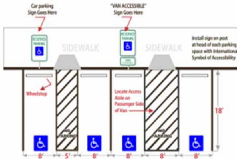
OPTION 1 - ACCESSIBLE PARKING Car Parking space 8' wide minimum with access aisle 5' wide Van parking Space 8' wide minimum with access aisle 8' wide
